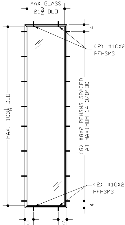
DOOR GLAZING
