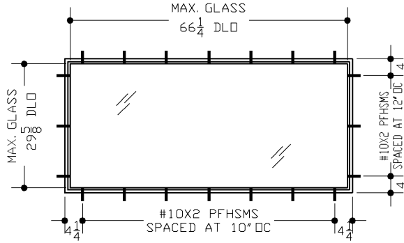
TRANSOM GLAZING
