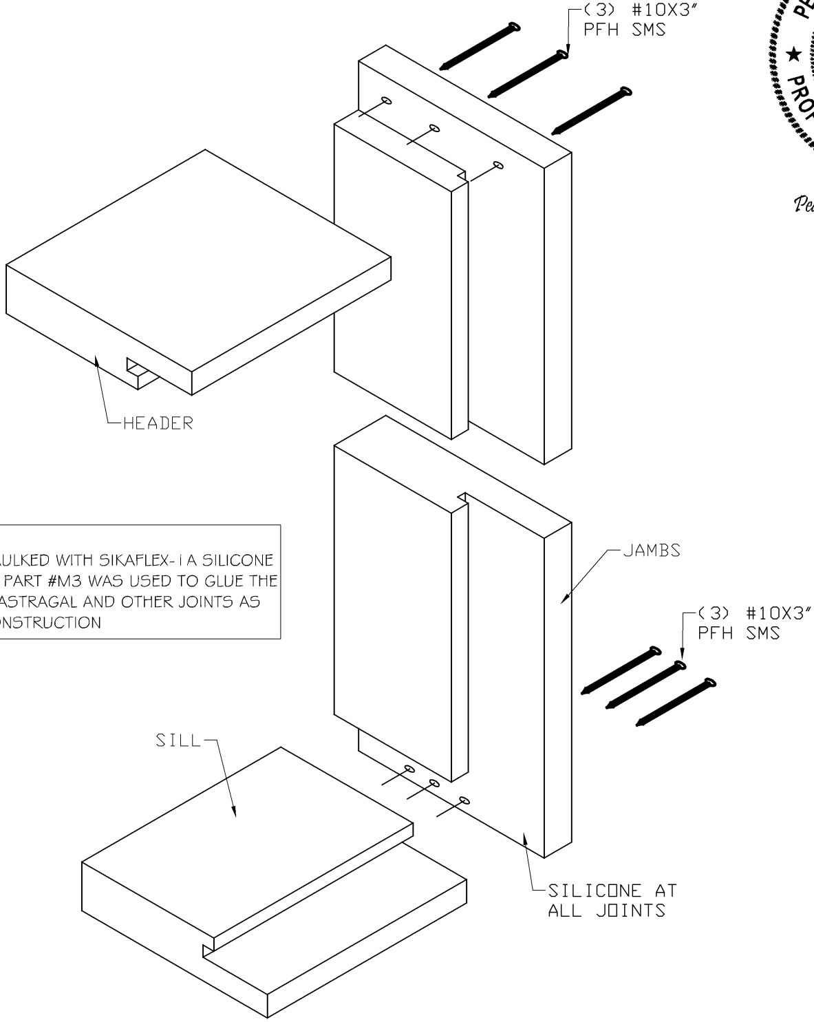
FRAME CONSTRUCTION:
