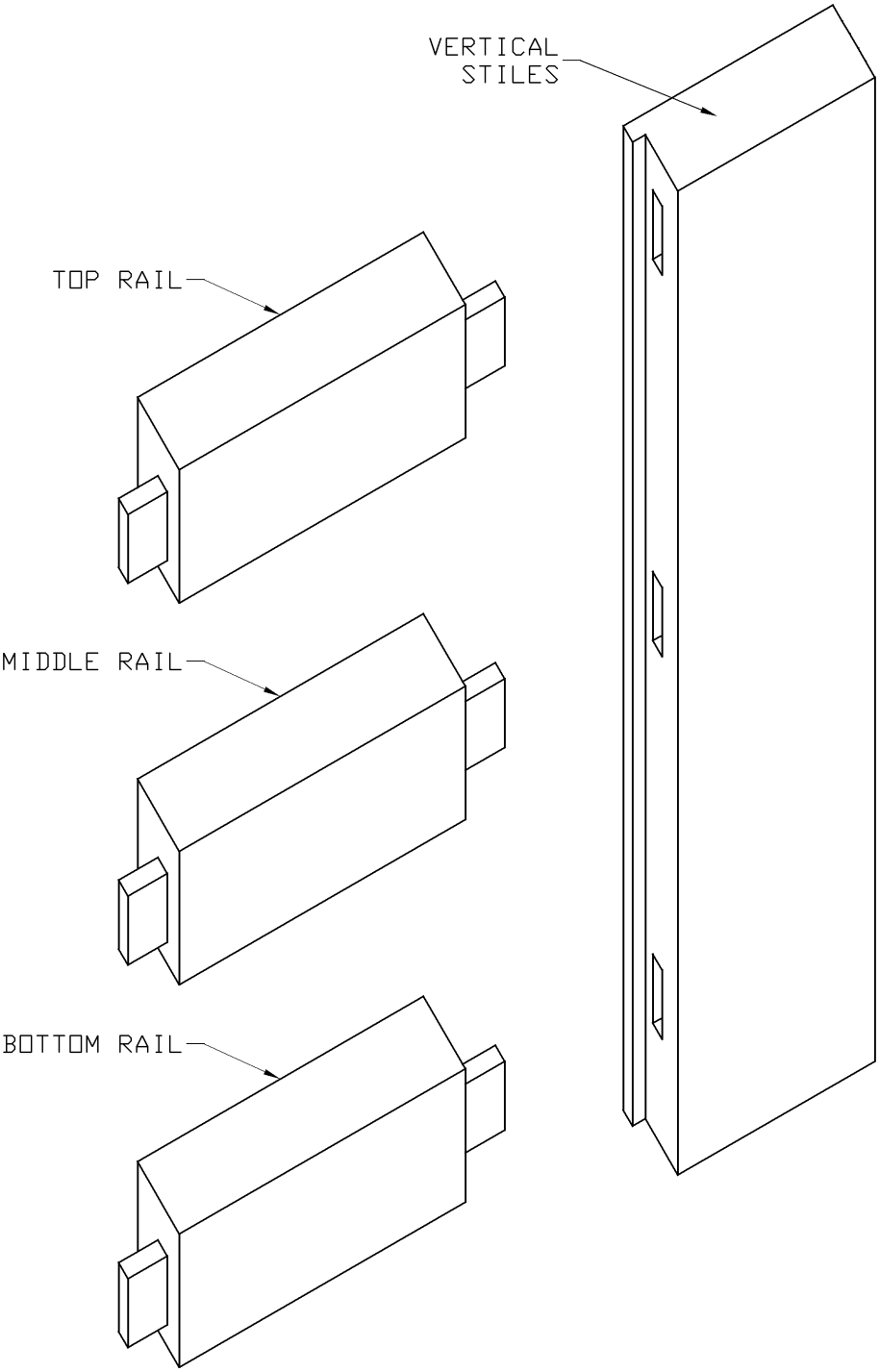
SASH CONSTRUCTION:
