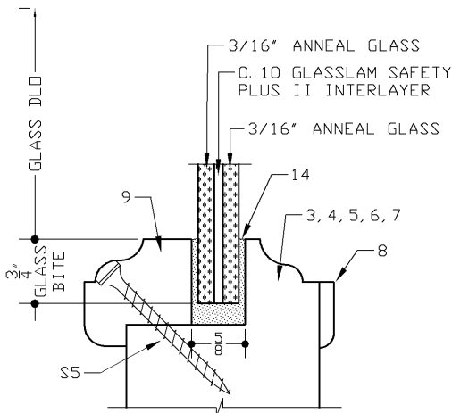
GLAZING DETAILS
